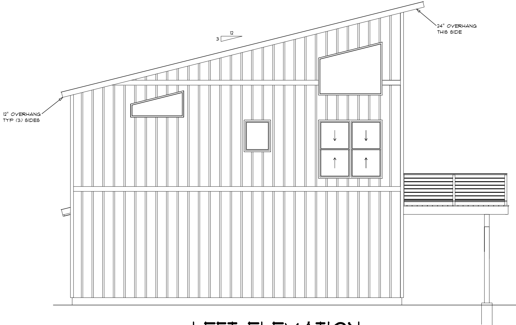
LEFT ELEVATION SCALE: 3/16" = 1'-0"
